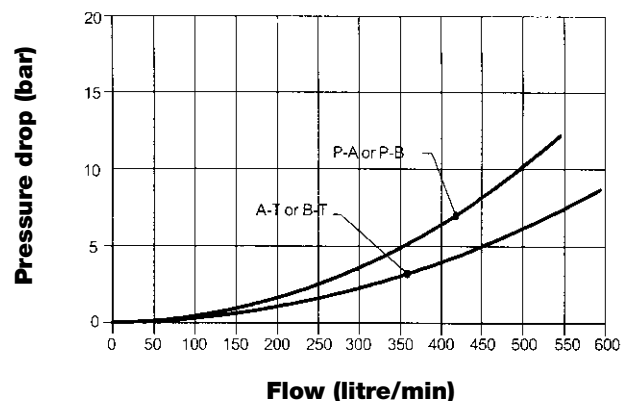
Pressure drop P-A/B-T spools selected
