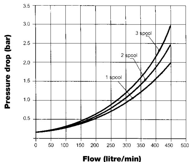
Pressure drop P-T spools in neutral
